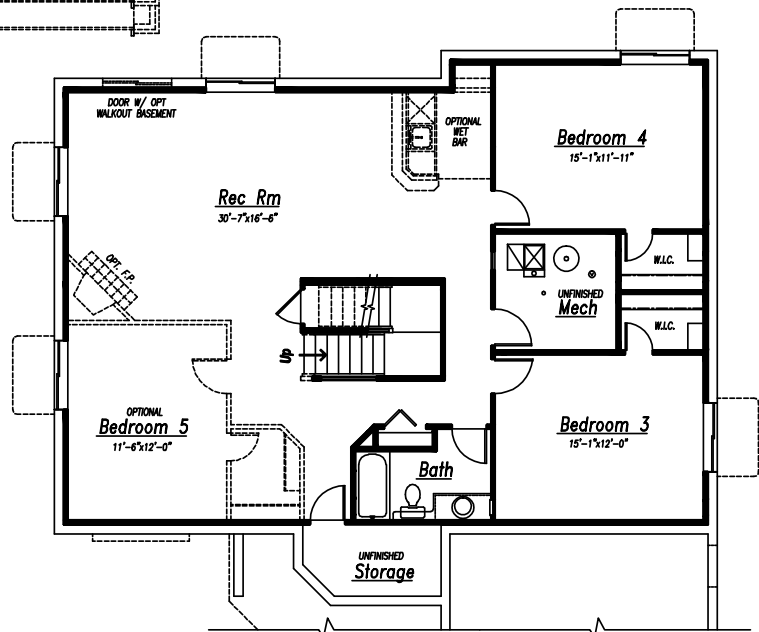
Basement Plan 1544 SQFT OPTIONAL FINISHED BASEMENT 1679 SQFT OPTIONAL UNFINISHED BASEMENT
