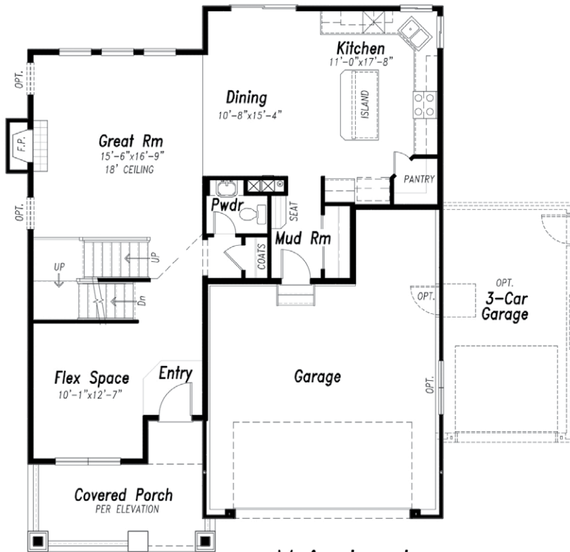
Main Level 1099 SQ FT
