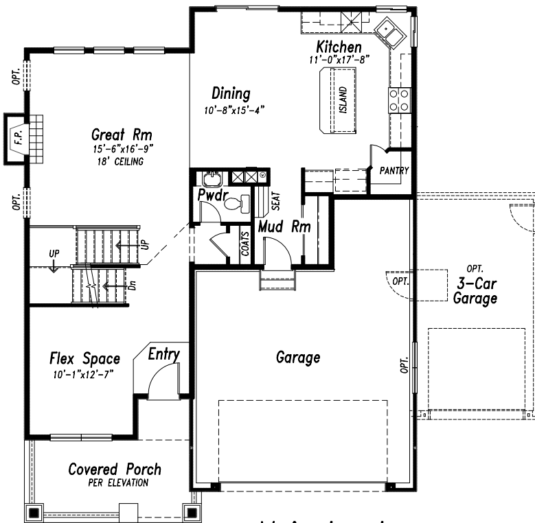
Main Level 1099 SQ FT
