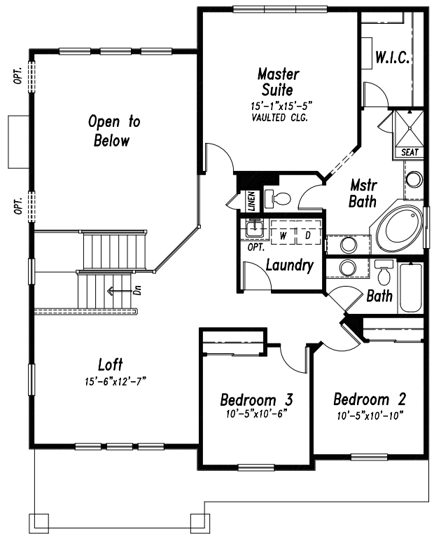
Upper Level 1198 SQ FT
