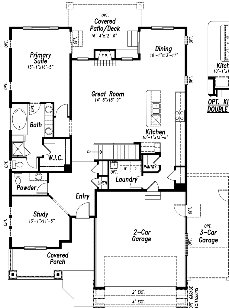
Main Level
